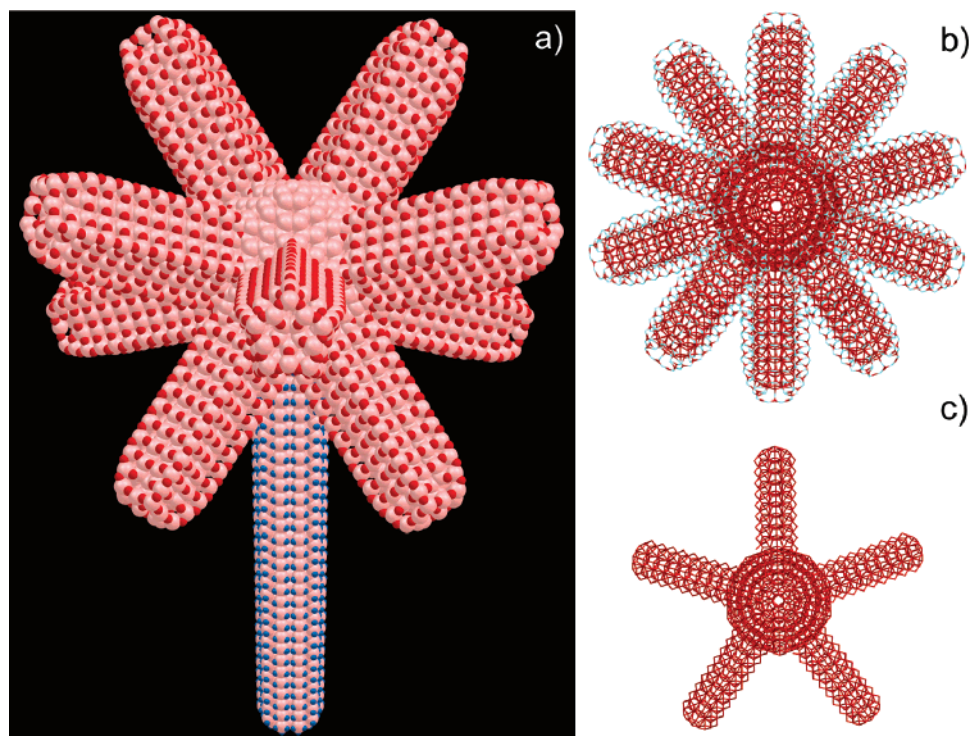
Figure 2. (a) SiNF with 10 petals covered by oxidized layers (oxygen atoms are in red and silicon atoms are in pink) and the stalk covered by hydrogen atoms (in blue). The petals and the stalk are attached to the SiIQD1100. (b) SiNF with 10 petals covered by an oxidized layer. The silicon atoms are in burgundy, and oxygen atoms are in green. (c) Silicon nanoflower with 5 petals.
