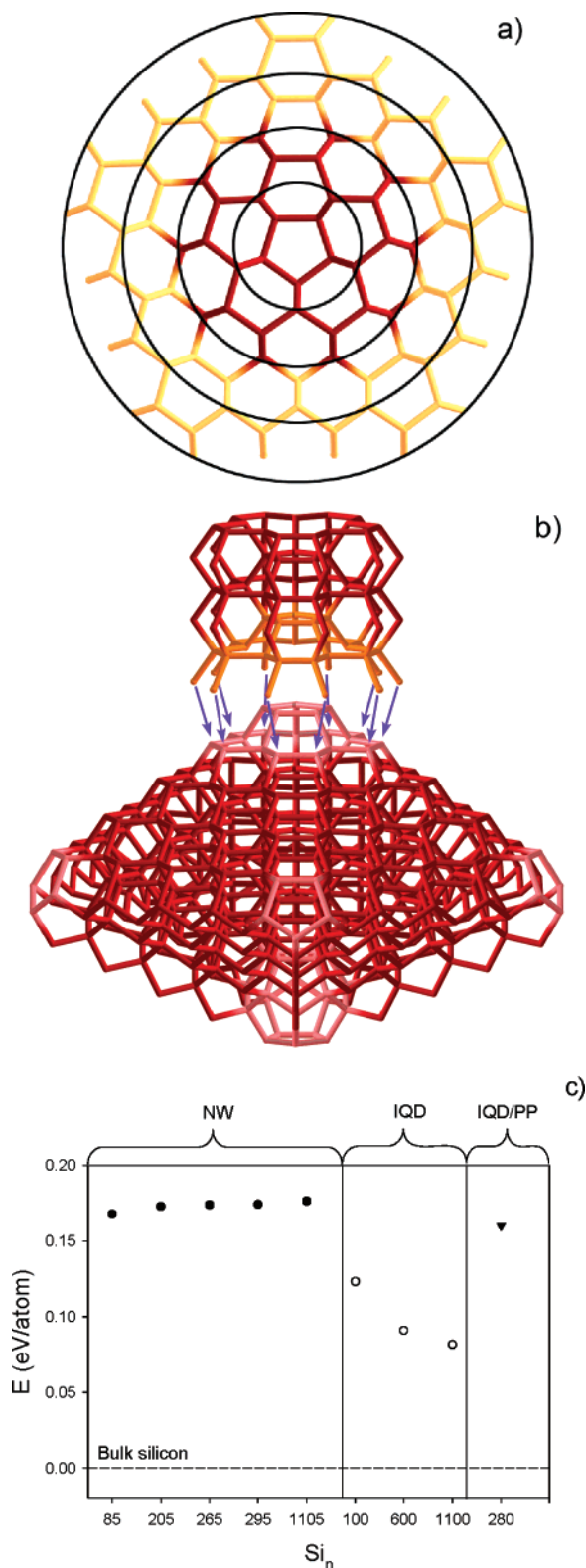
Figure 1. (a) Perpendicular cross section of the SiNW. The SiNW(1) part is in burgundy. (b) Atomic structure of IQD/PP interface (IQD is presented partially). The silicon atoms of the icosahedral core forming the pentagon vertexes are presented in pink. The PP atoms forming the IQD/PP interface are presented in orange. Blue arrows represent the chemical bonds between IQD and PP. (c) Relative stability (eV/atom, MM+ level of theory) of the different types of silicon nanostructures (dark and light circles are the SiNW and IQD energies, respectively, triangle is the IQD/PP energy) with respect to the MM+ binding energy of the bulk silicon (0.0 eV/atom).
